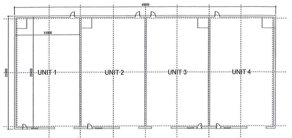
TYPICAL PLAN 1:200 2600 SQ FT UNITS
